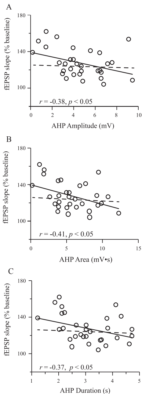
Fig. 5. Synaptic plasticity is correlated with intrinsic excitability. The magnitude of LTP was significantly correlated with the amplitude (A), area (B), and duration (C) of the post-burst AHP (solid lines). Data are mean values for each animal where both intrinsic excitability and synaptic plasticity were studied in the same slice. Interestingly, when good learners are removed from the plot, the correlation is no longer significant (dashed line indicates slope of the line in the absence of good learners). Abbreviations: long-term potentiation (LTP); after-hyperpolarization (AHP).
